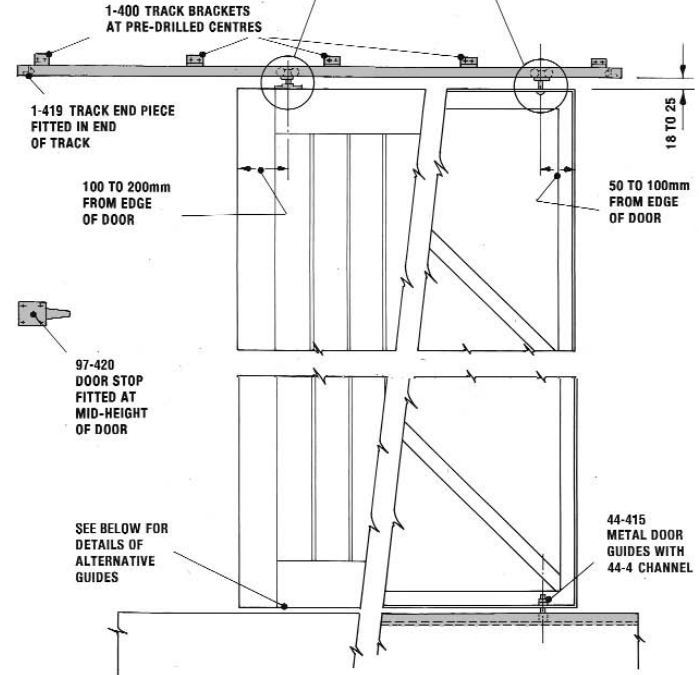
ELEVATION OF TIMBER AND METAL DOORS
