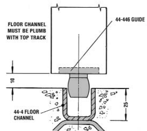
TIMBER DOORS OVER 1500MM WIDE
